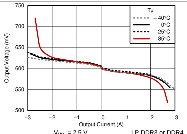
Figure 10. Load Regulation
