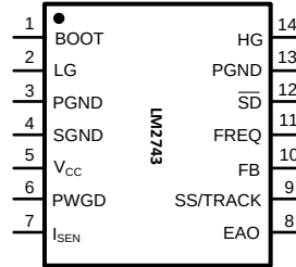
Pin Functions
