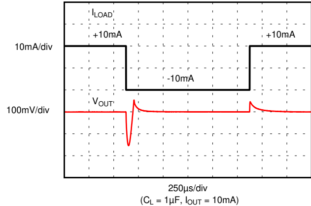
Figure 8. Load Transient
