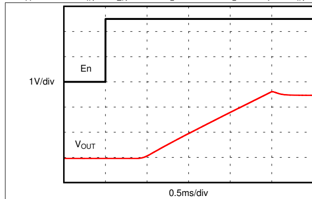
Figure 13. Turnon Time (Enable)
