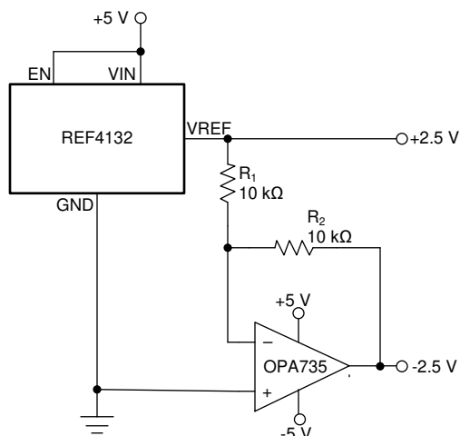
Simplified Schematic
