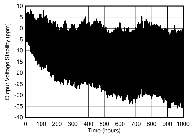
Figure 14. Long Term Stability - 1000 hours ( V_{REF} )
