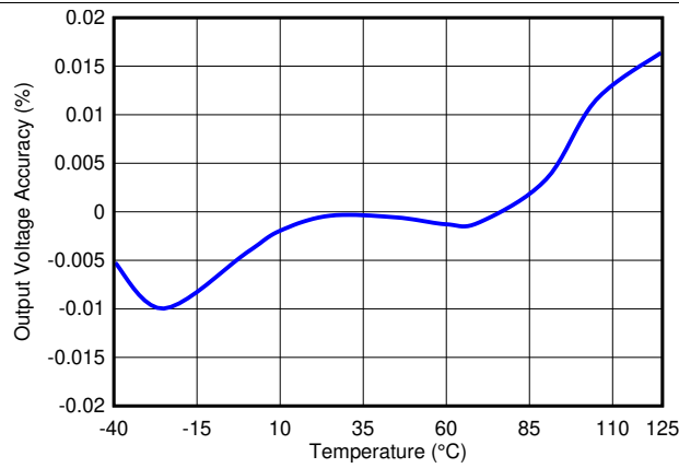
Figure 1. Output Voltage Accuracy vs Temperature
