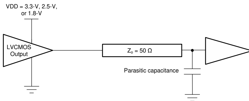
图 7-3. Application Load With Termination
