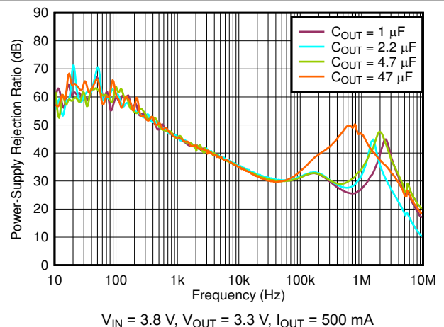
图 6-42. PSRR vs Frequency and C_{OUT}
