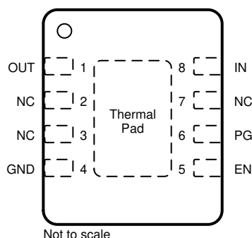
图 5-4. DRB Package, 8-Pin Fixed VSON (Top View)
