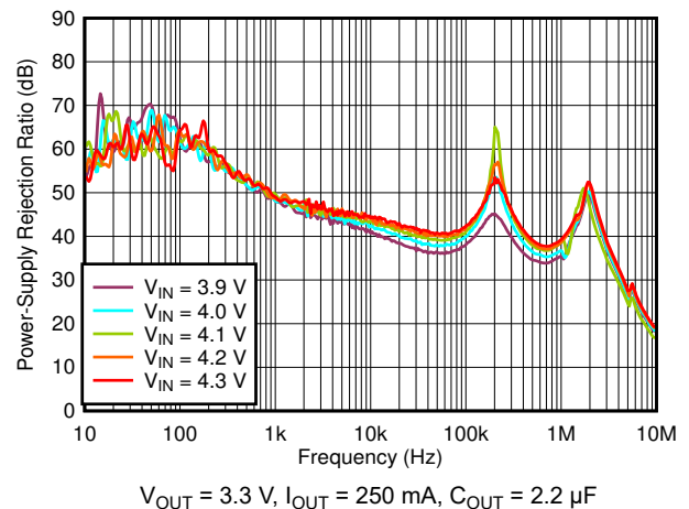
图 6-40. PSRR vs Frequency and V_{IN}
