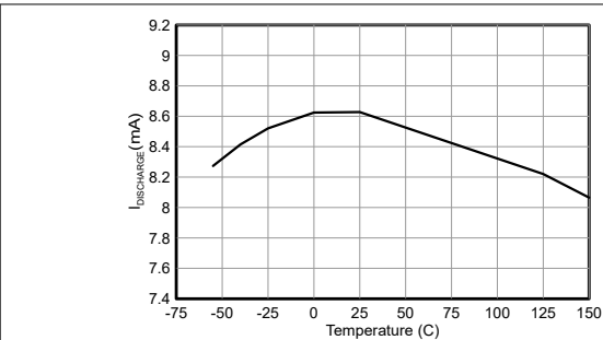
图 5-1. Oscillator Discharge Current vs Temperature for V_{IN} = 15\text{ V} and V_{OSC} = 2\text{ V}
