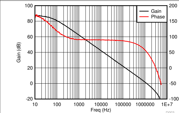
图 5-3. Error Amplifier Open-Loop Gain and Phase vs Frequency V_{CC} = 15\text{ V} , R_L = 100\text{ k}\Omega , and T_A = 25^\circ\text{C}
