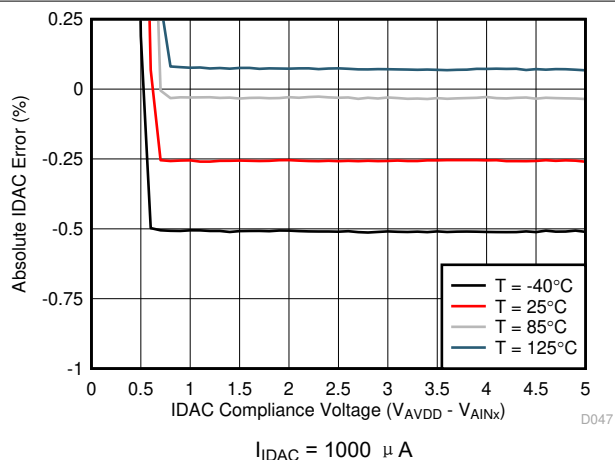
图 7-39. IDAC Error vs Compliance Voltage
