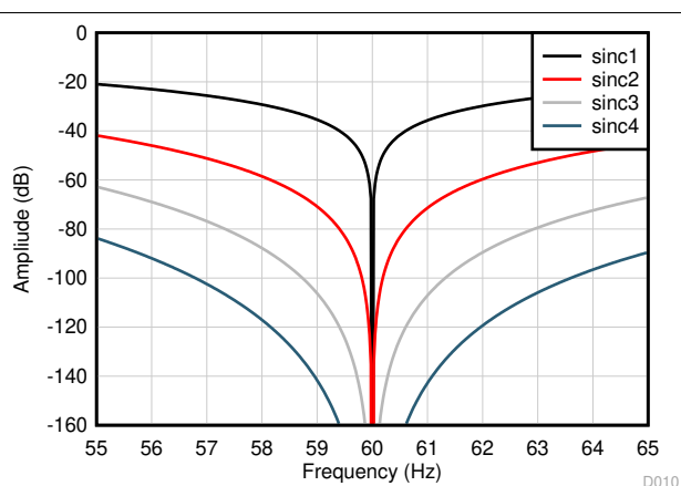
图 9-21. Sinc Frequency Response Zoom (60 SPS)
