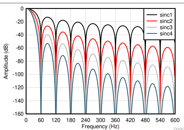
图 9-19. Sinc Frequency Response (60 SPS)
