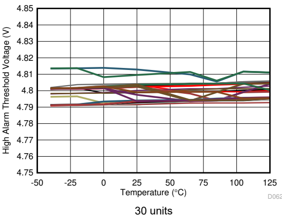
图 7-48. ADC1 Absolute High Alarm Threshold vs Temperature
