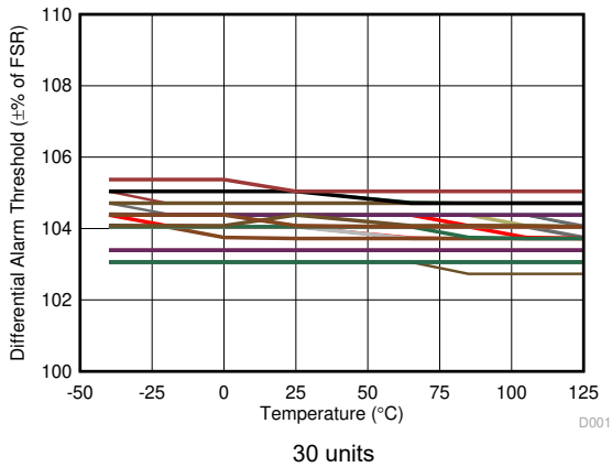
图 7-46. ADC1 Differential Over-range Alarm Threshold vs Temperature
