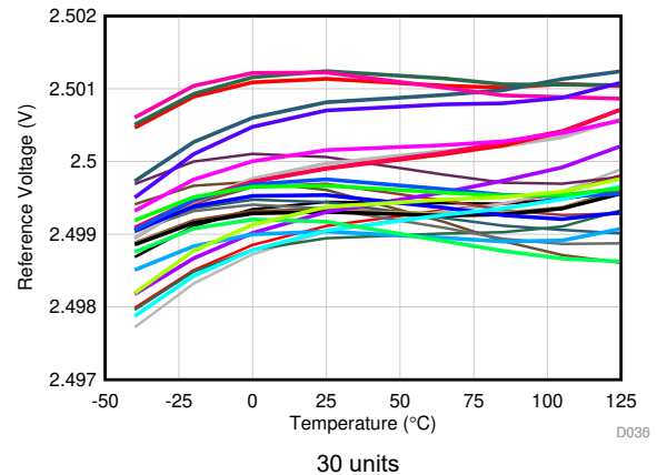
图 7-31. Voltage Reference vs Temperature
