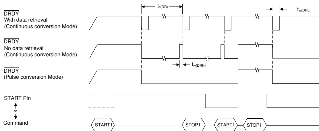
图 9-42. \overline{\text{DRDY}} Operation
