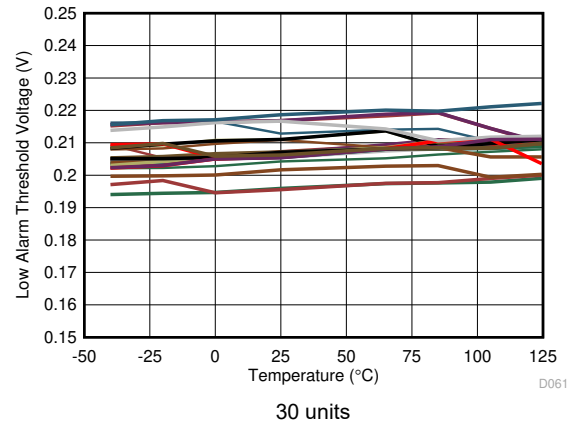
图 7-47. ADC1 Absolute Low Alarm Threshold vs Temperature
