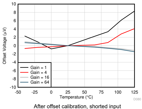
图 7-50. ADC2 Offset Voltage vs Temperature
