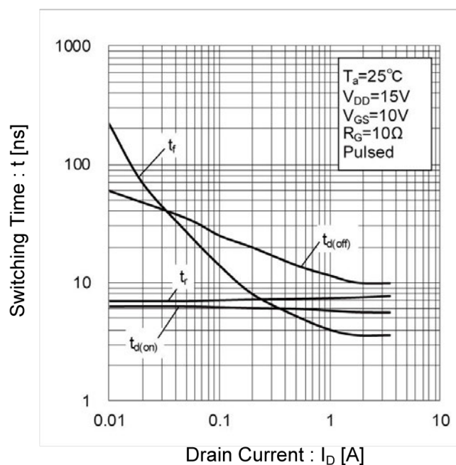
Fig.13 Switching Characteristics
