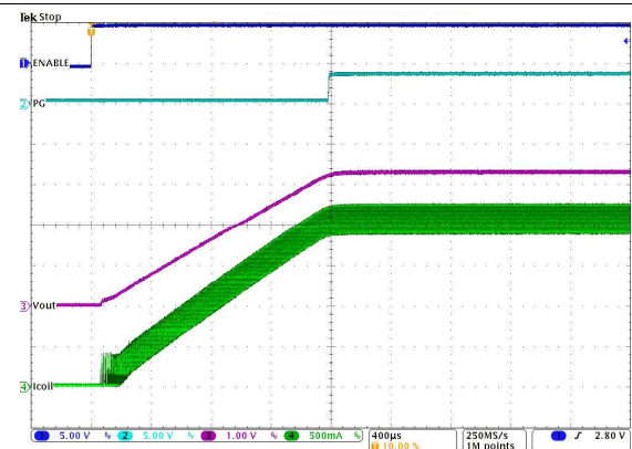
Figure 42. Start Up into 3 A
