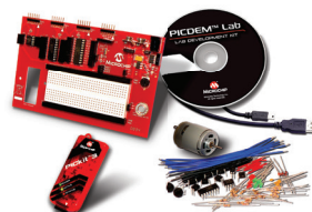
PICDEM™ Lab Development Kit (DM163045)
