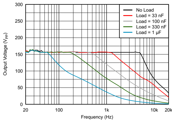
图 6-9. Gain Bandwidth at V_{PVDD} = 30 \text{ V}
