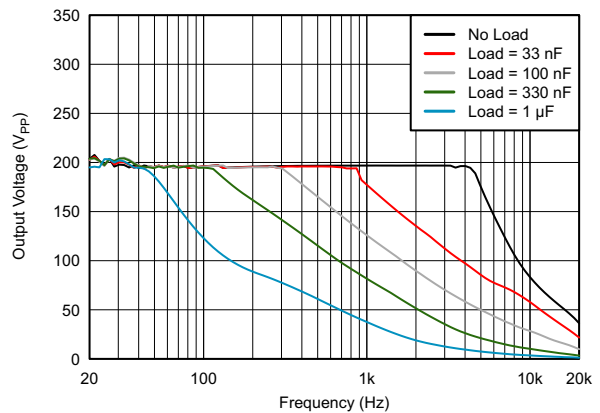
图 6-10. Gain Bandwidth at V_{PVDD} = 55 \text{ V}
