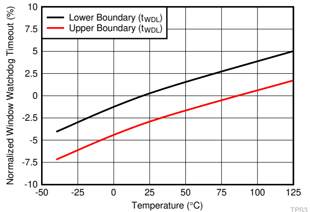
图 6-7. Normalized Watchdog Timeout Accuracy Over Temperature (SET0 = 1, SET1 = 1, CWD = 10kΩ to VDD)
