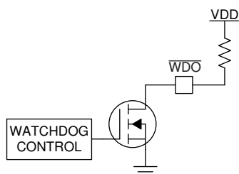
图 8-7. Open-Drain \overline{\text{WDO}} Configuration
