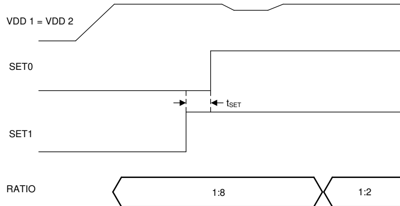
图 7-4. Changing SET0 and SET1 Pins
