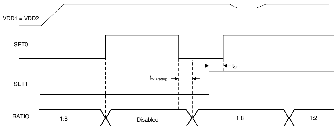
图 6-3. Changing SET0 and SET1 Pins
