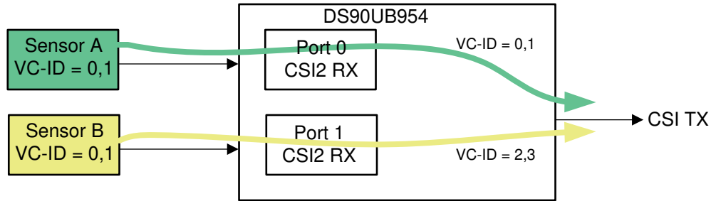
Figure 7-13. VC-ID Mapping Example 2
