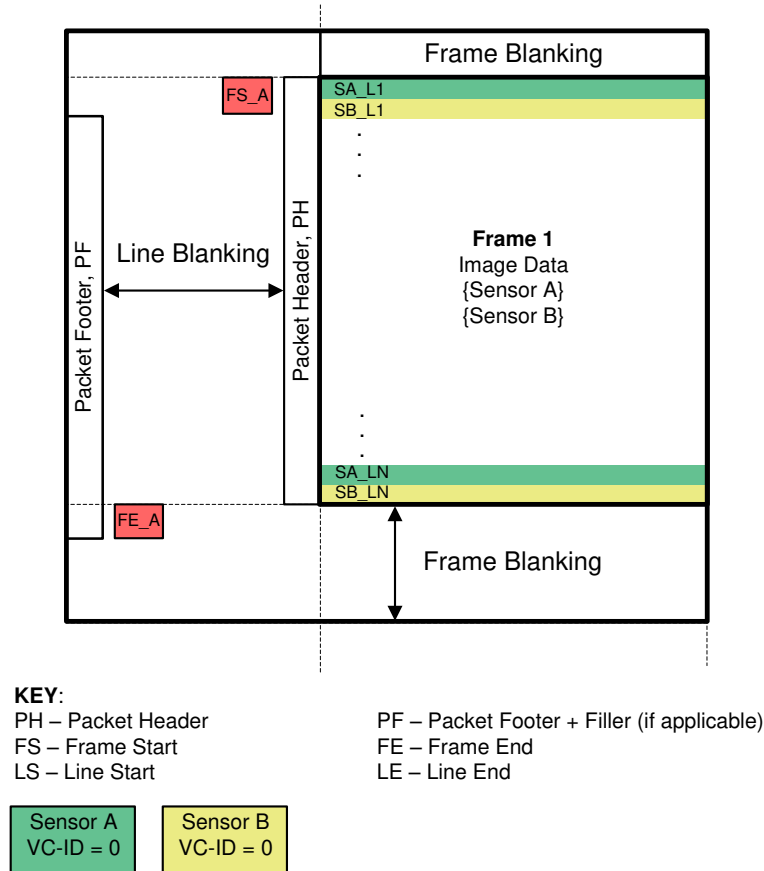
Figure 7-22. Line-Interleave Format
