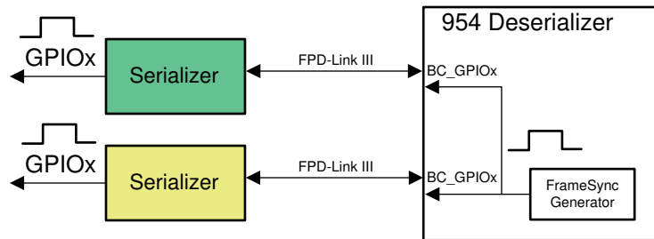
Figure 7-19. Internal FrameSync
