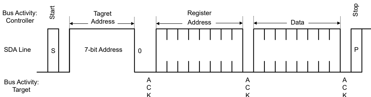
Figure 7-27. Serial Control Bus — WRITE
