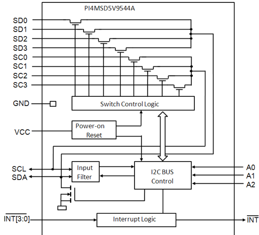
Figure 1: Block Diagram
