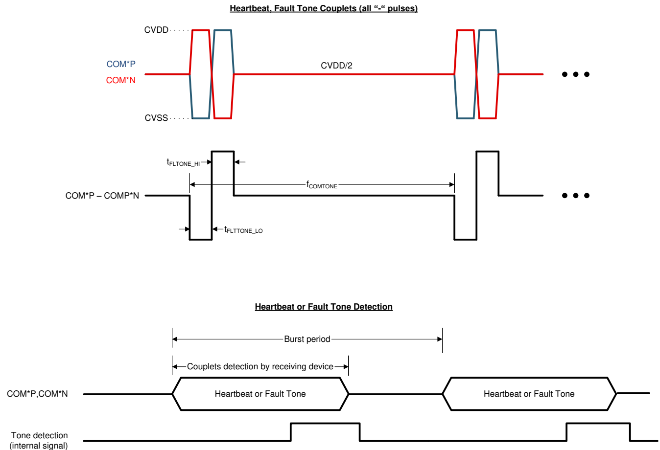
图 9-45. Heartbeat and Fault Tone
