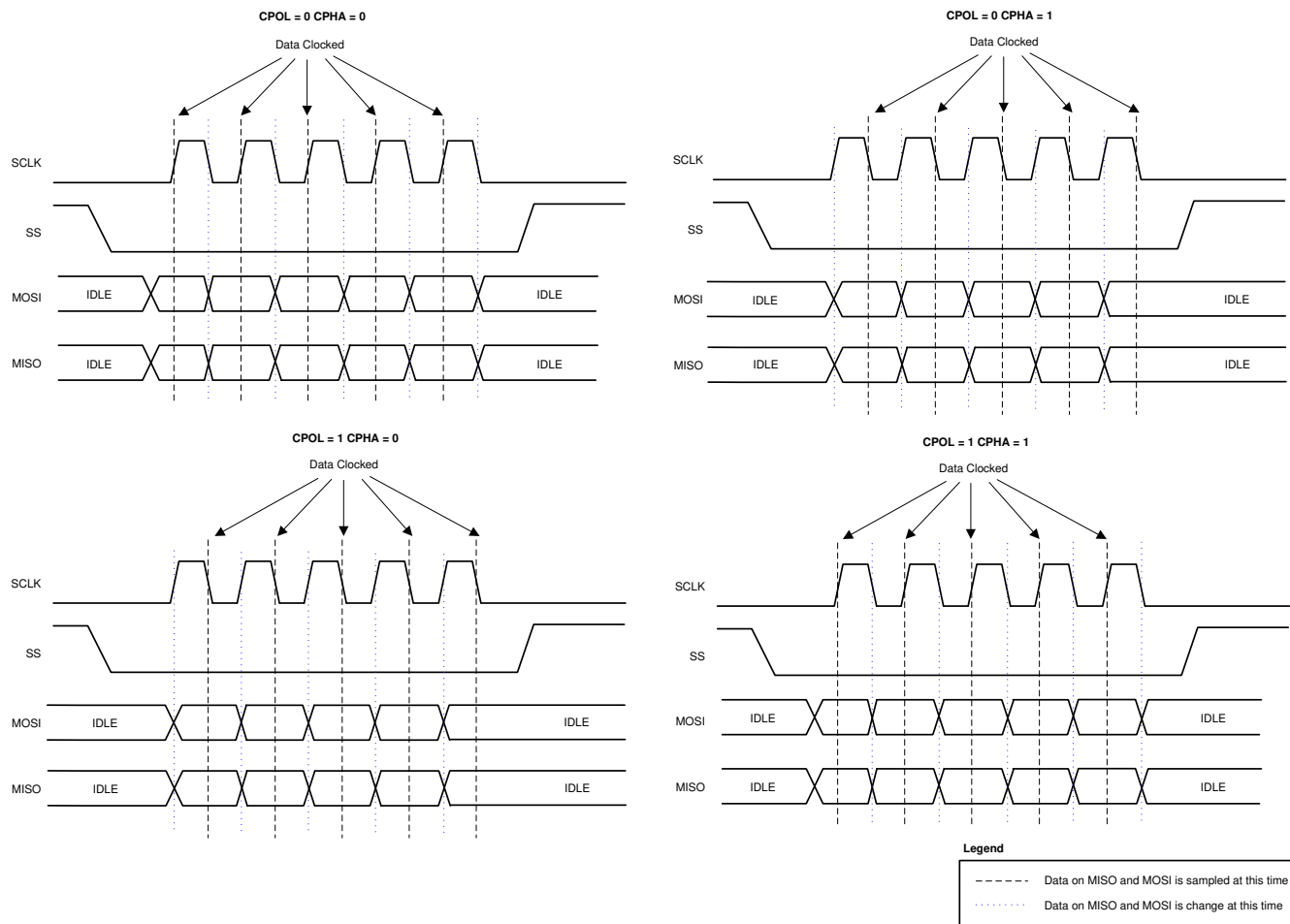
图 9-40. SPI Master CPOL and CPHA
