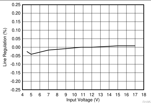
图 7-6. Line Regulation, I_{OUT} = 6\text{ A}
