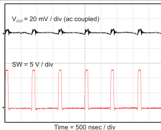
图 7-13. Output Voltage Ripple, I_{OUT} = 12 \text{ A}
