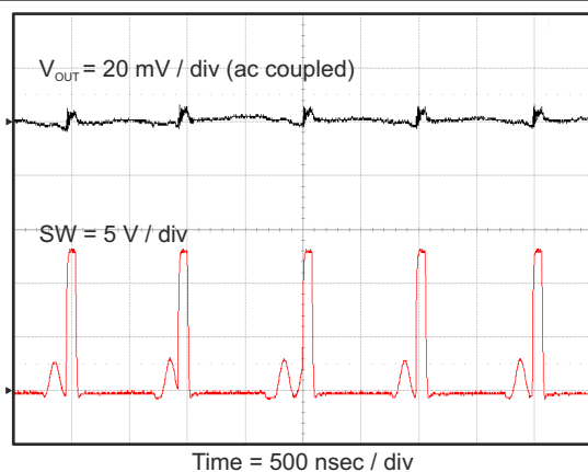
图 7-12. Output Voltage Ripple, I_{OUT} = 800 \text{ mA}
