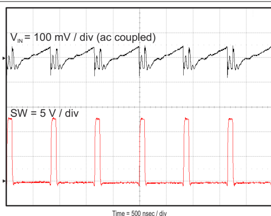
图 7-10. Input Voltage Ripple, I_{OUT} = 12 \text{ A}
