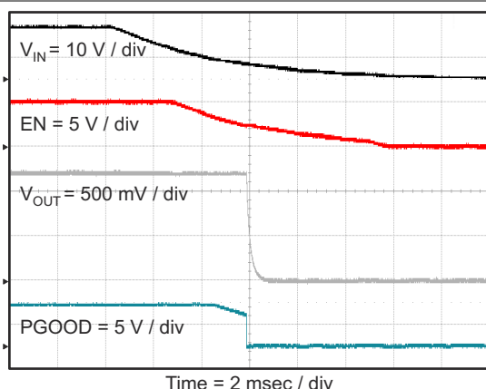
图 7-16. Shut Down Relative to V_{IN} Falling
