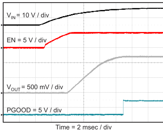
图 7-14. Start Up Relative to V_{IN} Rising
