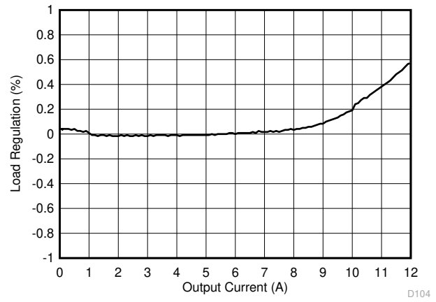
图 7-5. Load Regulation, V_{IN} = 12\text{ V}
