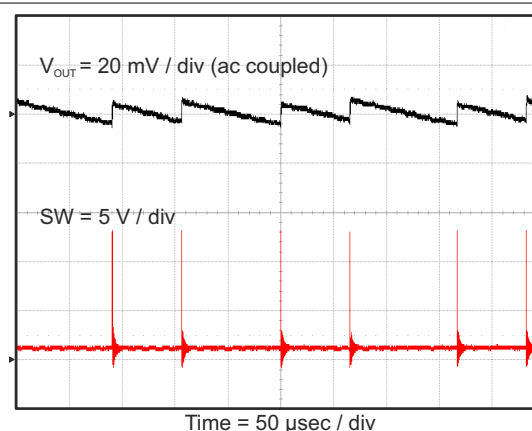
图 7-11. Output Voltage Ripple, I_{OUT} = 10 \text{ mA}
