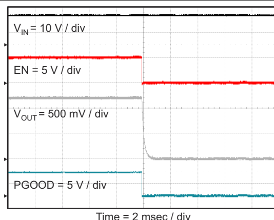
图 7-17. Shut Down Relative to EN Falling
