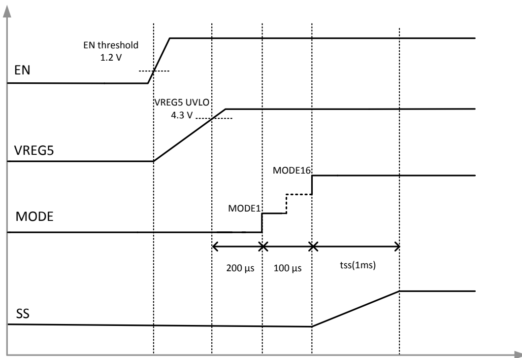
图 6-2. Power-Up Sequence
