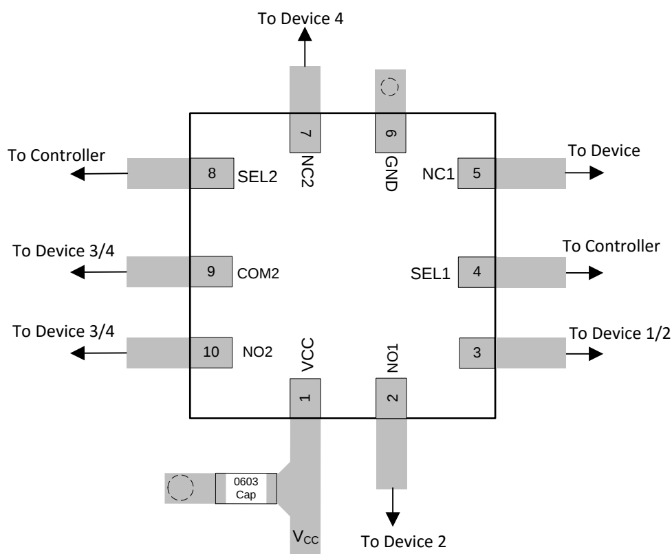
Figure 15. Layout Example
