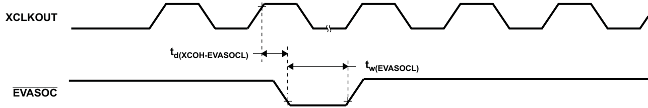
Figure 5-17. \overline{EVASOC} Timing
