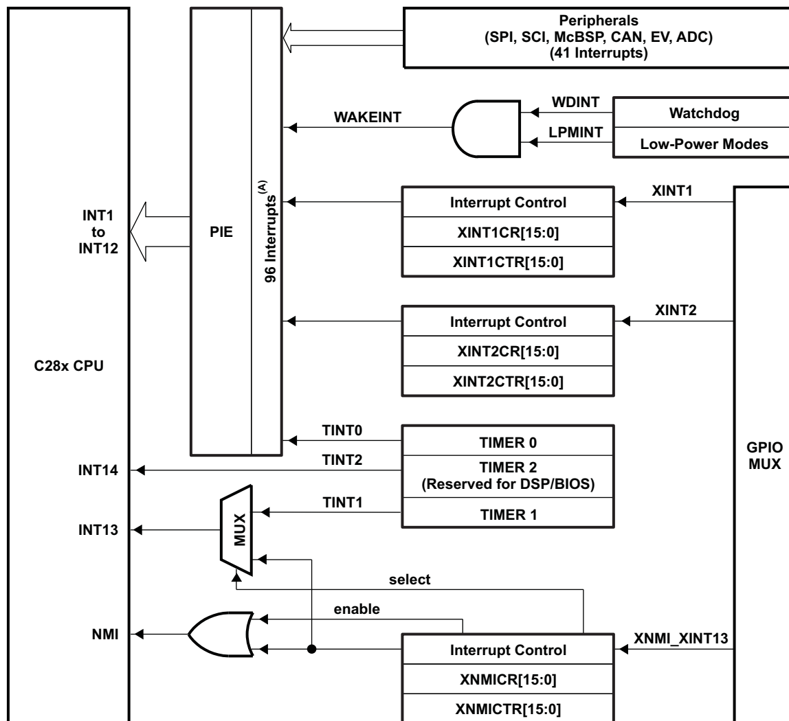
Figure 6-17. Interrupt Sources
