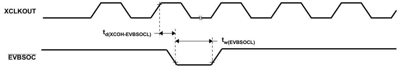
Figure 5-18. \overline{EVBSOC} Timing
