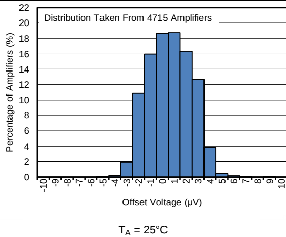
Figure 1. Offset Voltage Production Distribution at 25^\circ\text{C}
