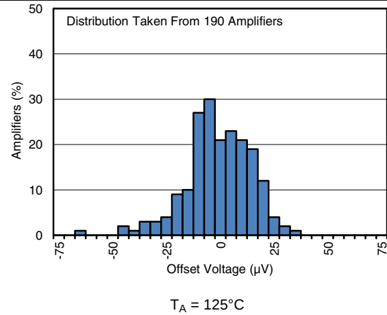
Figure 2. Offset Voltage Production Distribution at 125^\circ\text{C}
