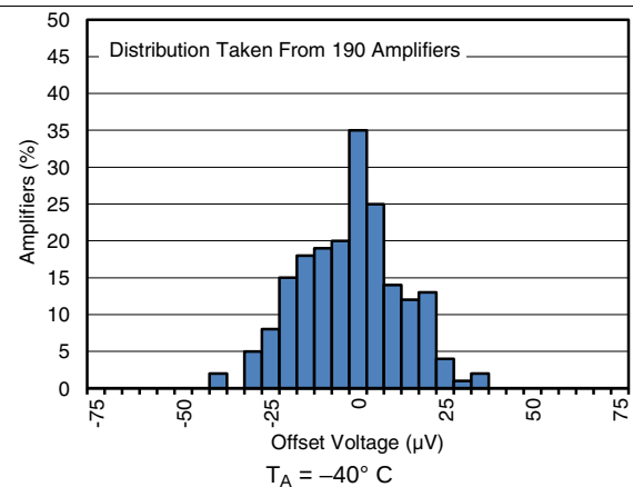
Figure 6. Offset Voltage Production Distribution at -40^\circ\text{C}
