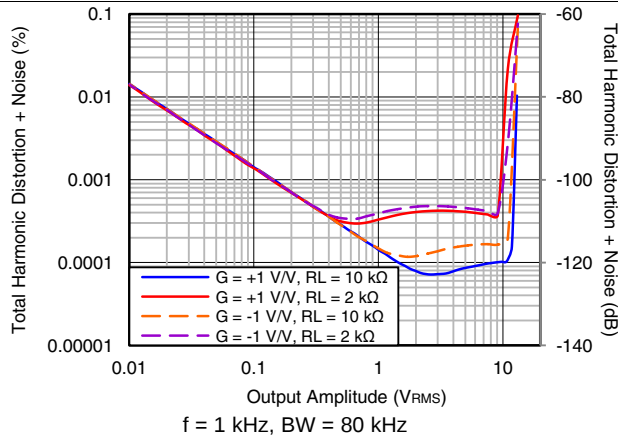
Figure 25. THD+N vs Output Amplitude
