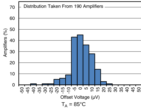
Figure 3. Offset Voltage Production Distribution at 85^\circ\text{C}
