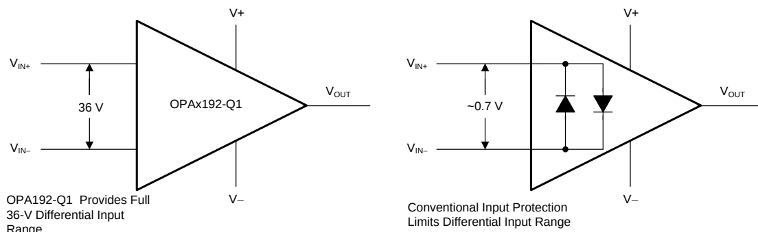
Figure 49. OPAx192-Q1 Input Protection Does Not Limit Differential Input Capability
