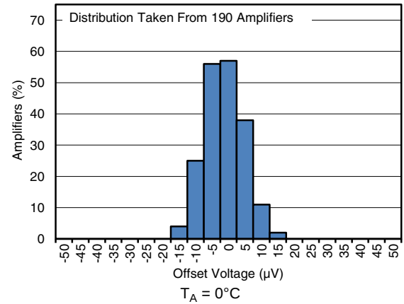
Figure 4. Offset Voltage Production Distribution at 0^\circ\text{C}
