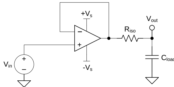
Figure 57. Extending Capacitive Load Drive with the OPAx192-Q1
