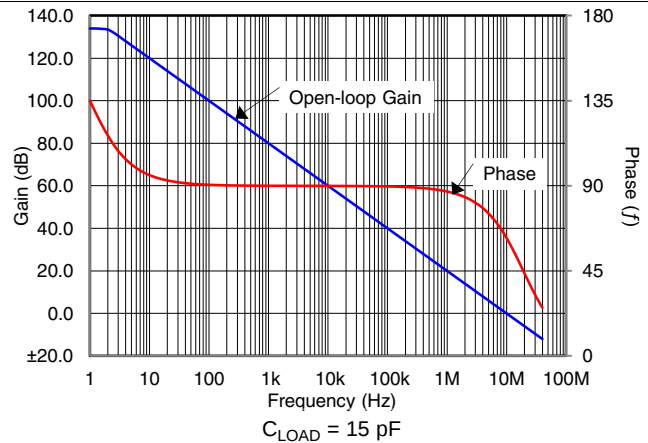
Figure 14. Open-Loop Gain and Phase vs Frequency
