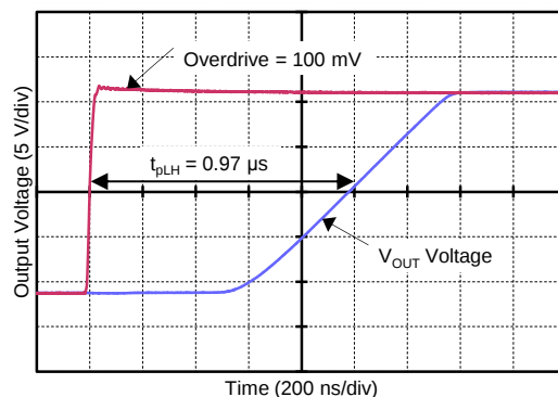
Figure 44. Propagation Delay Rising Edge
