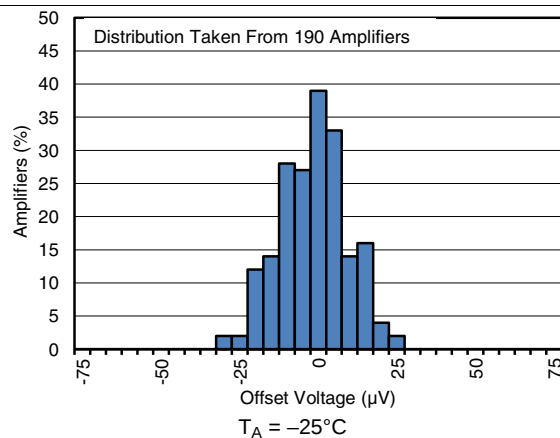
Figure 5. Offset Voltage Production Distribution at -25^\circ\text{C}
