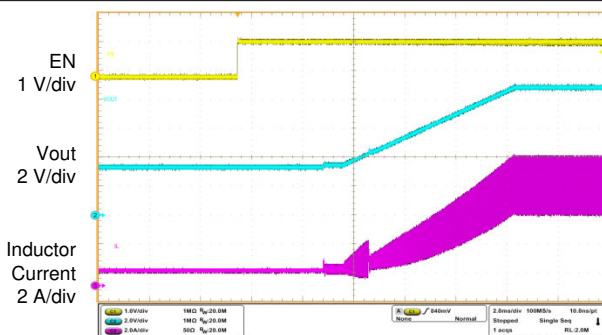
图 8-5. Startup Waveforms
