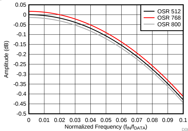
Figure 50. Non-Binary OSR \text{Sinc}^3 Filter Frequency Response
