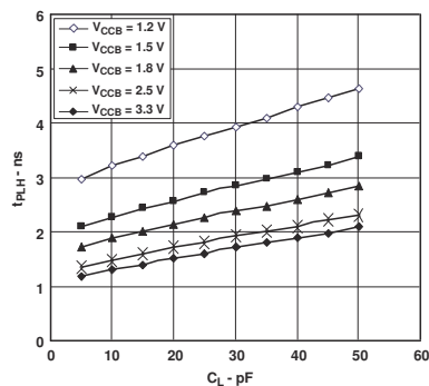
图 5-5. Typical A-to-B Propagation Delay, Low to High
