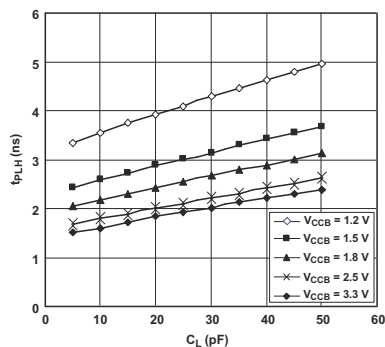
图 5-1. Typical A-to-B Propagation Delay, Low to High
