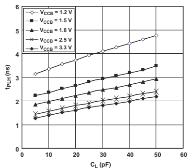
图 5-3. Typical A-to-B Propagation Delay, Low to High
