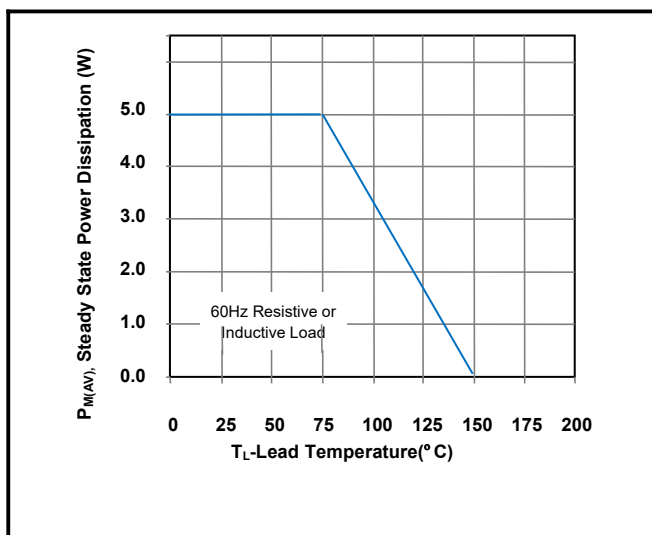
Figure 6 - Steady State Power Derating Curve
