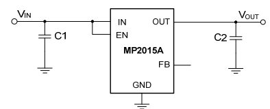
Output Fixed Version (QFN)
