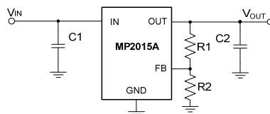
Output Adjustable Version (TSOT)
