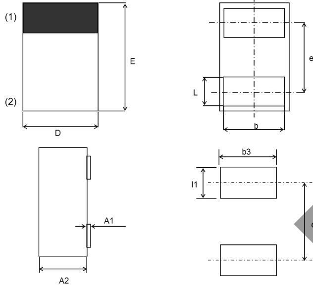
DFN1006-2, (VML2)
